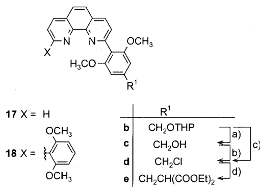
Figure 1. a) p TsOH, EtOH; b) conc. HCl; c) conc. HCl; d) CH 2 (COOEt) 2 , NaH, DMF; THP = tetrahydropyran-2-yl
